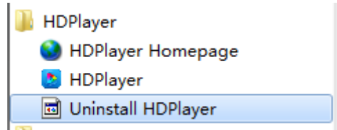
图 1-6 Software Uninstall
