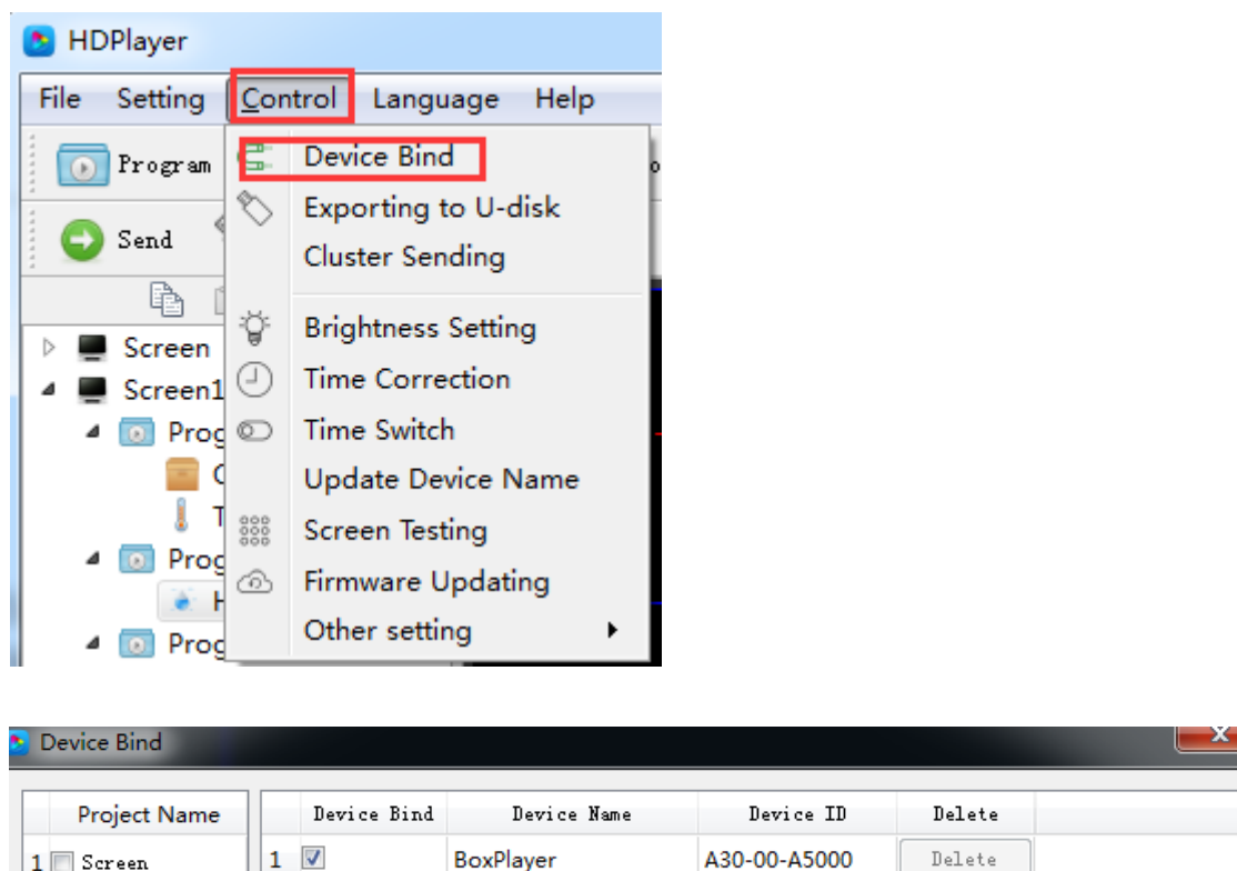
Fig. 6-1 Device Bind
