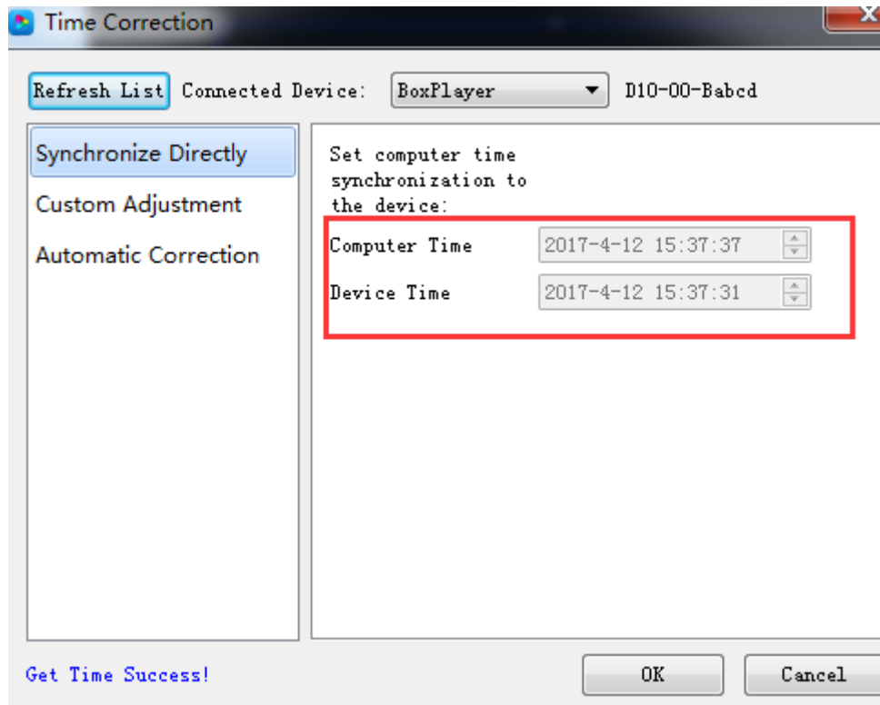
Fig.6-5 Synchronous Correction
