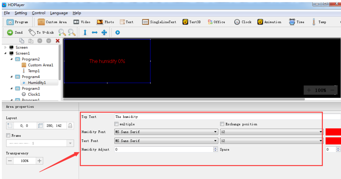
Fig. 3-32 Humidity Attribute
