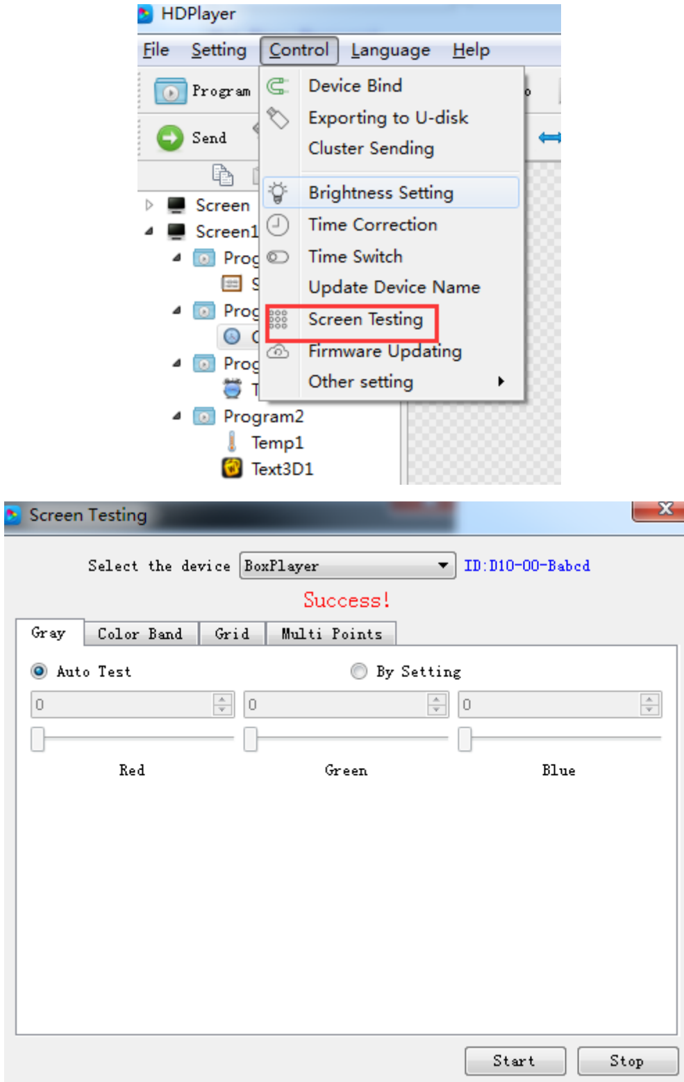
Fig. 6-7 Screen Testing
