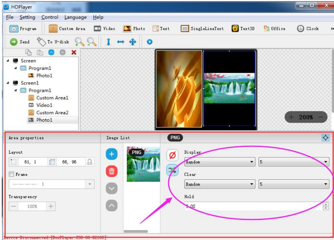
Fig. 3-11 Photo properties
