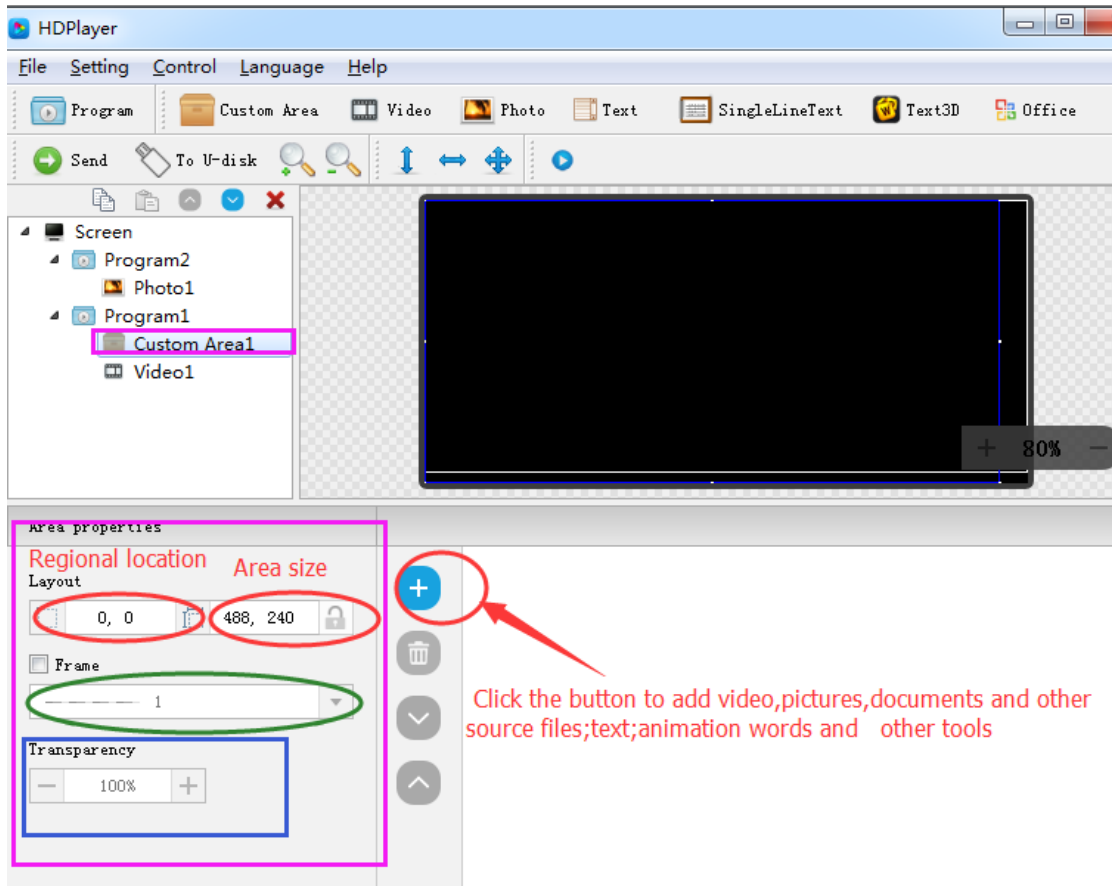
Fig. 3-8 Area attributes
