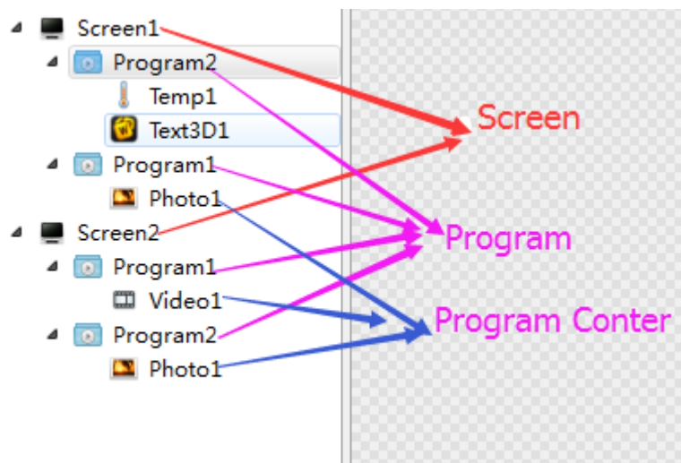
Fig.3-2 Program Structure
