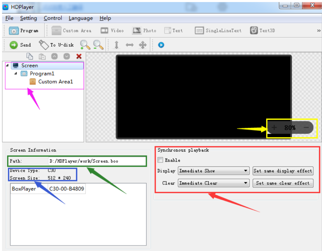
Fig. 3-4 Display properties
