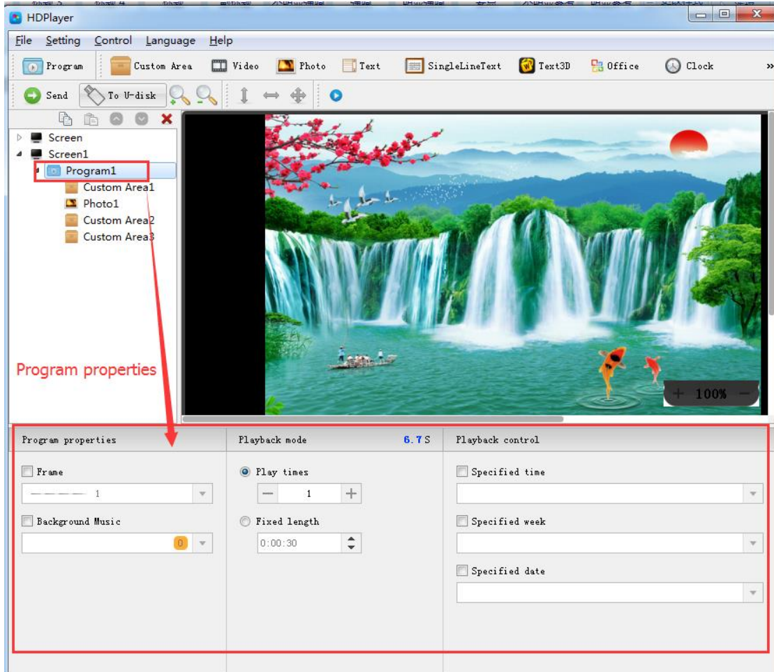
Fig. 3-6 Program attributes
