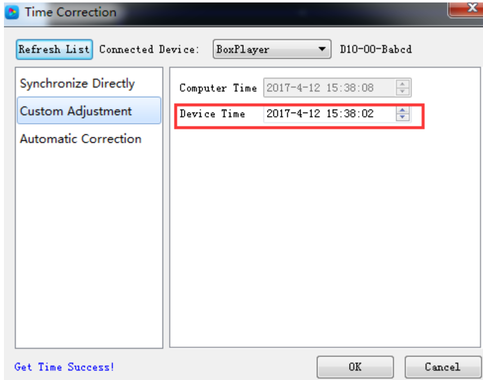
Fig. 6-6 Custom adjustment
