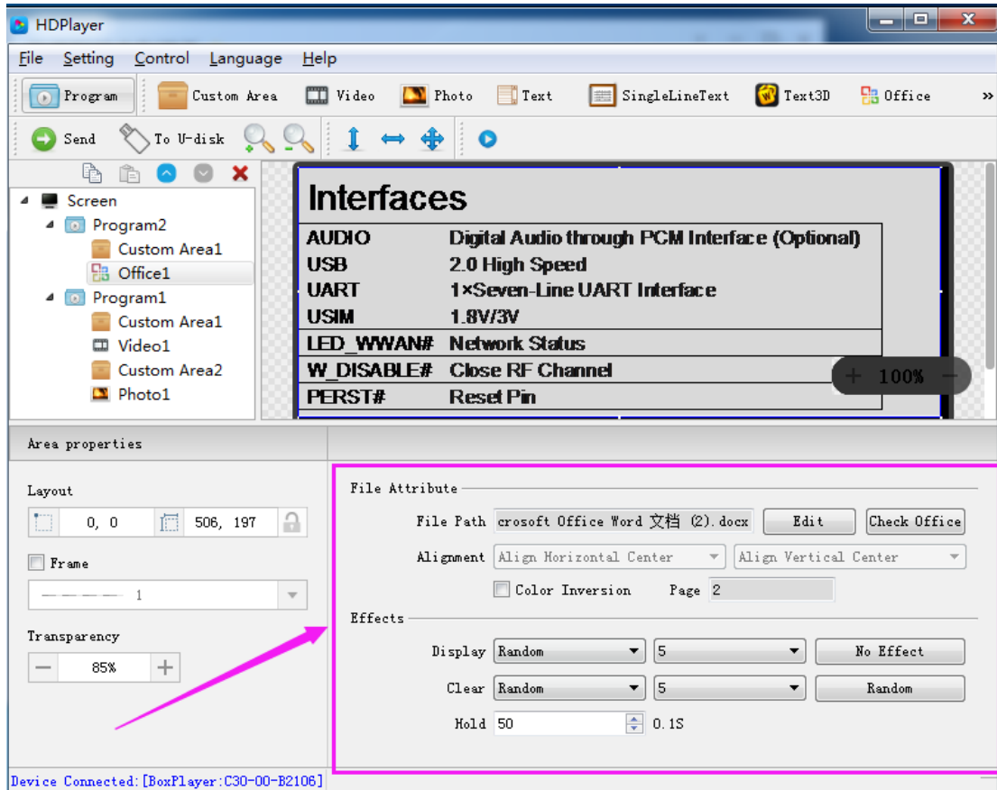
Fig. 3-13 File properties
