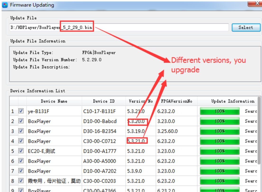
Fig. 6-8 Firmware Update
