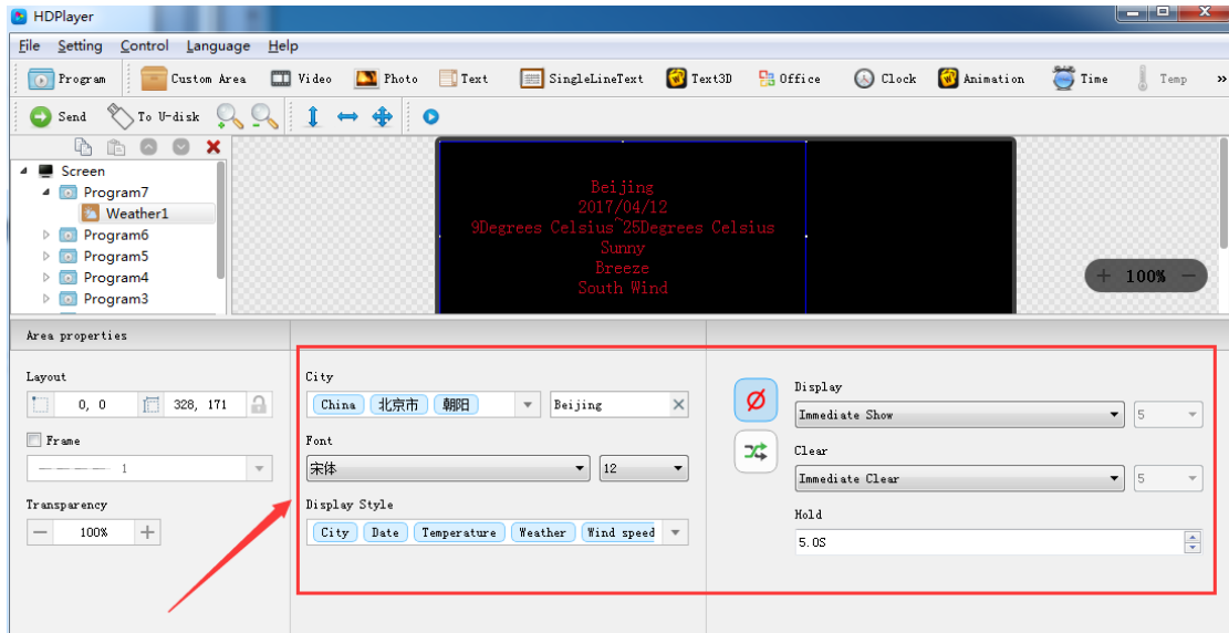
图 3-40 Weather Attribute
