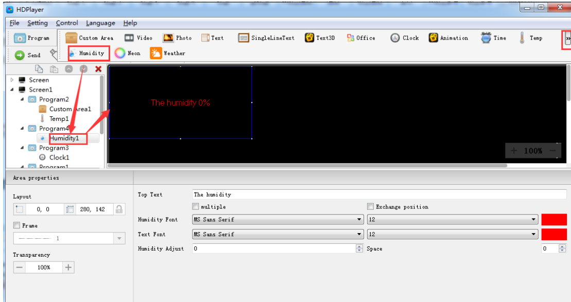
Fig. 3-31 Add Humidity
