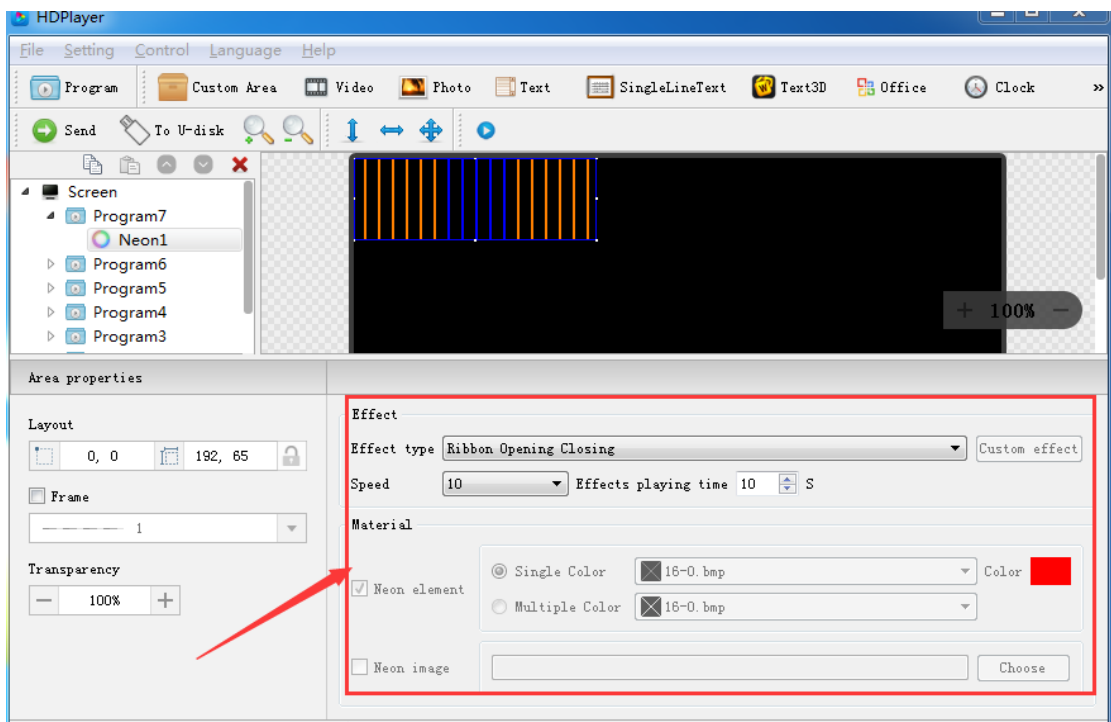
Fig. 3-34 Neon Attribute
